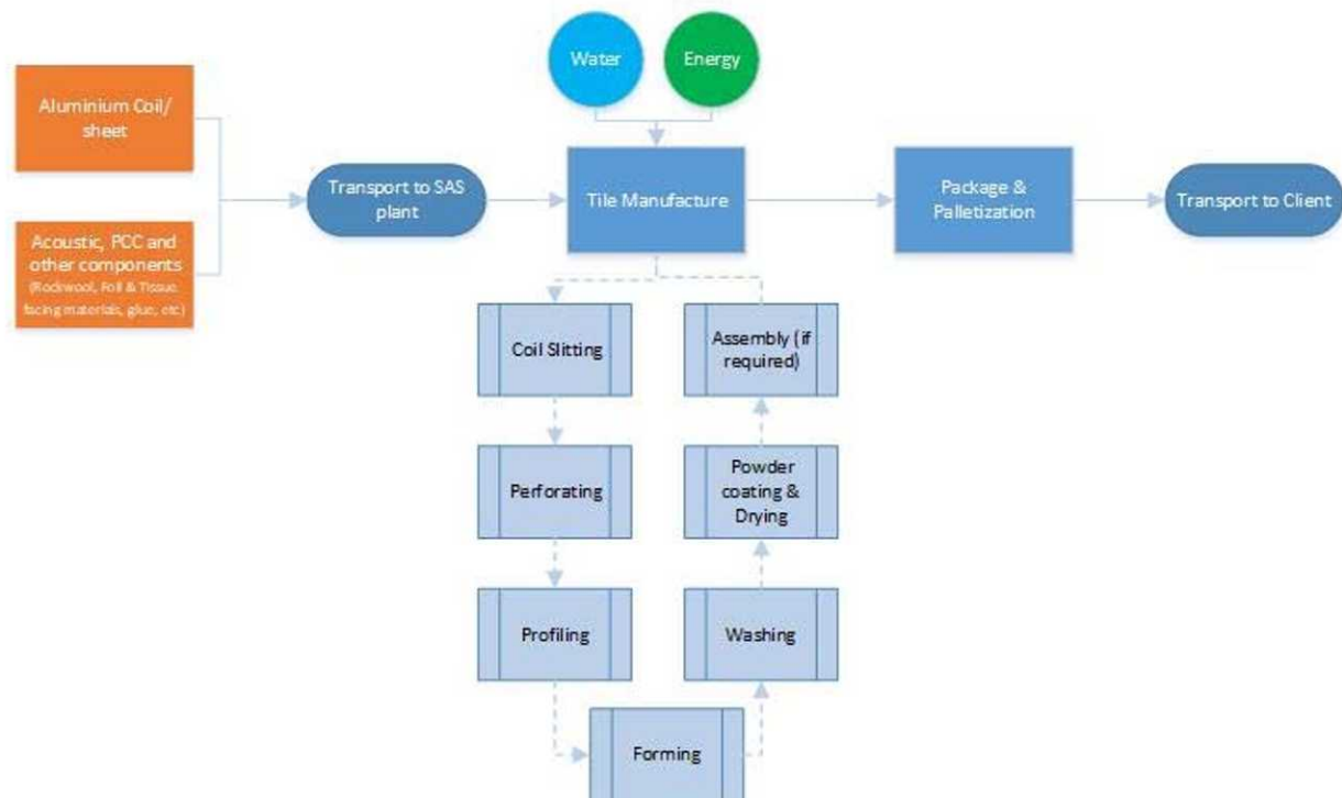
SAS Ceiling Aluminium Tile Manufacturing Process
