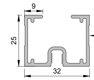
C-PROFILE SECTION
