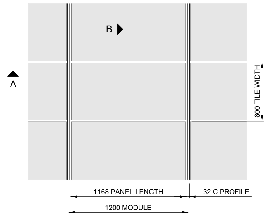
PART REFLECTED PLAN SCALE N.T.S.
