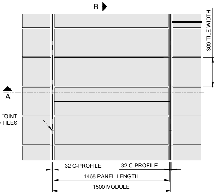
PART REFLECTED PLAN SCALE N.T.S.
