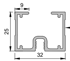
C-PROFILE SECTION
